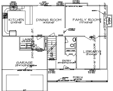
1 FIRST FLOOR PLAN A-3 SCALE: 1/4"=1'-0"
