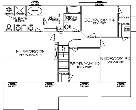
1 SECOND FLOOR PLAN A-4 SCALE: 1/4"=1'-0"
