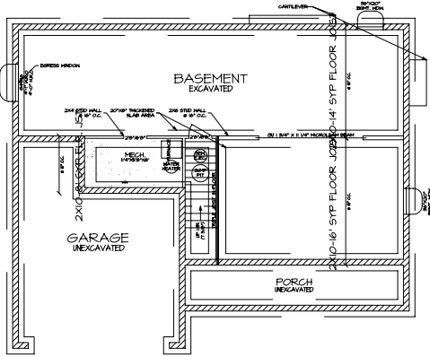
1 FOUNDATION PLAN A-2 SCALE: 1/4"=1'-0"
